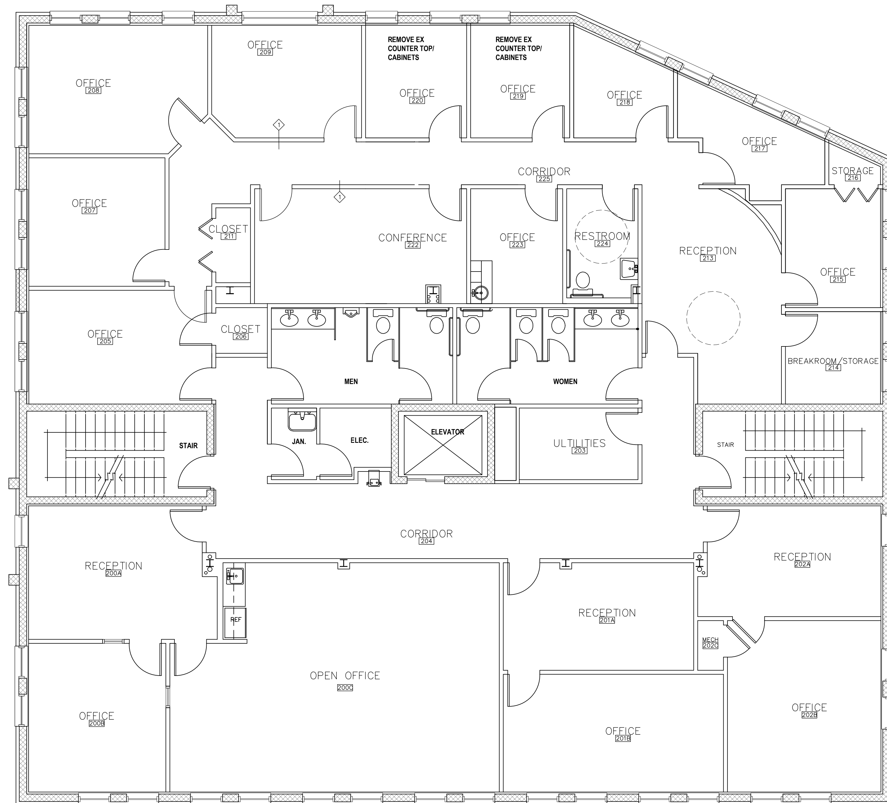
SECOND FLOOR PLAN SCALE : 3 / 16" = 1'-0"
